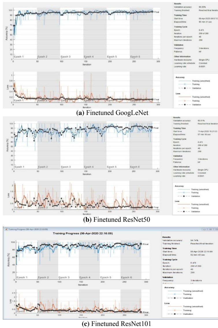
Fig. 4. Results of training and loss for various PTNs using SGDM
