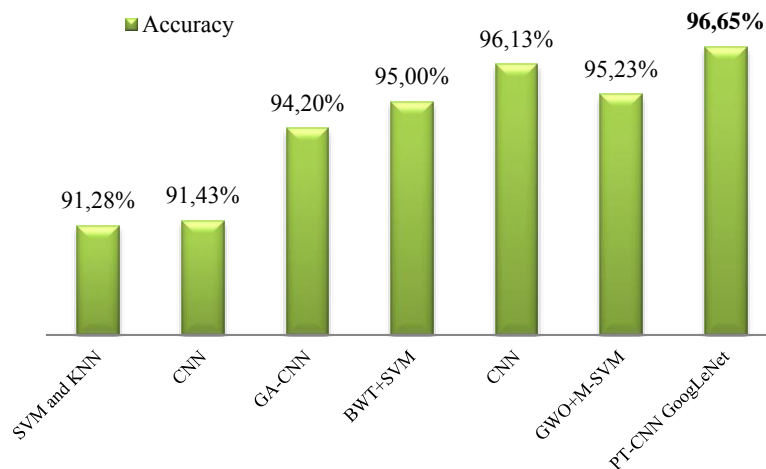
Fig. 6. Evaluation against the State of the Art
